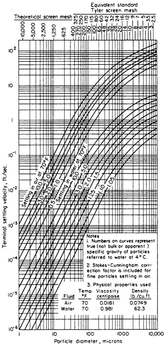
Fig. 5-82. Terminal velocities of spherical particles of different densities settling in air and water at 70°F. under the action of gravity. (From Lapple et al., op. cit. , p. 292.)
