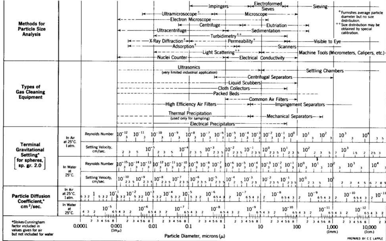
FIG. 1. Characteristics of particles and particle dispersoids. Reprinted by permission of Stanford Res. Inst. J. 5, 95 (1961).
