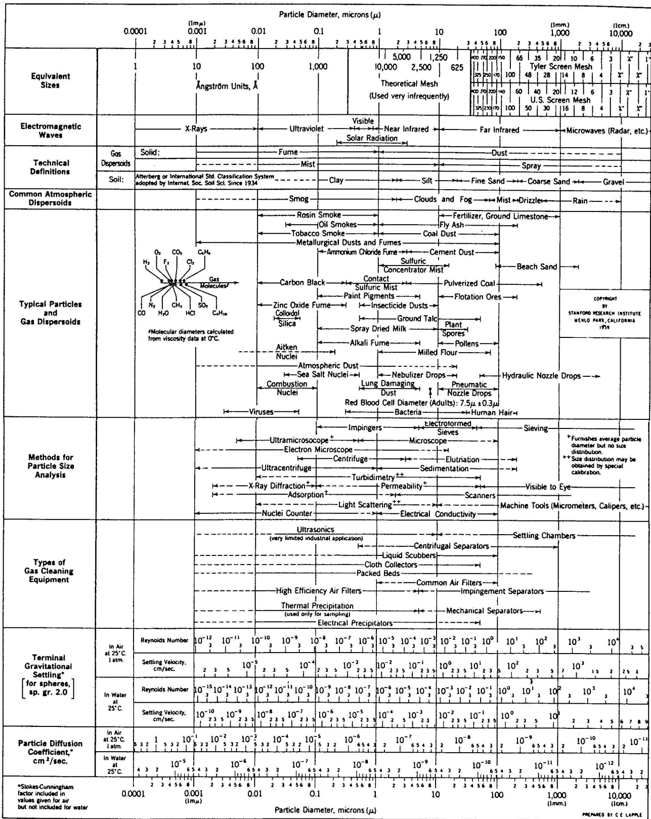
FIG. 1. Characteristics of particles and particle dispersoids. Reprinted by permission of Stanford Res. Inst. J. 5, 95 (1961).
