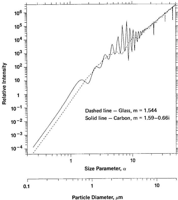
Figure 4-11. Relative intensity for I_1 + I_2 vs. size parameter and sphere diameter for illumination by a HeNe laser for particles with two different refractive indices, m .
