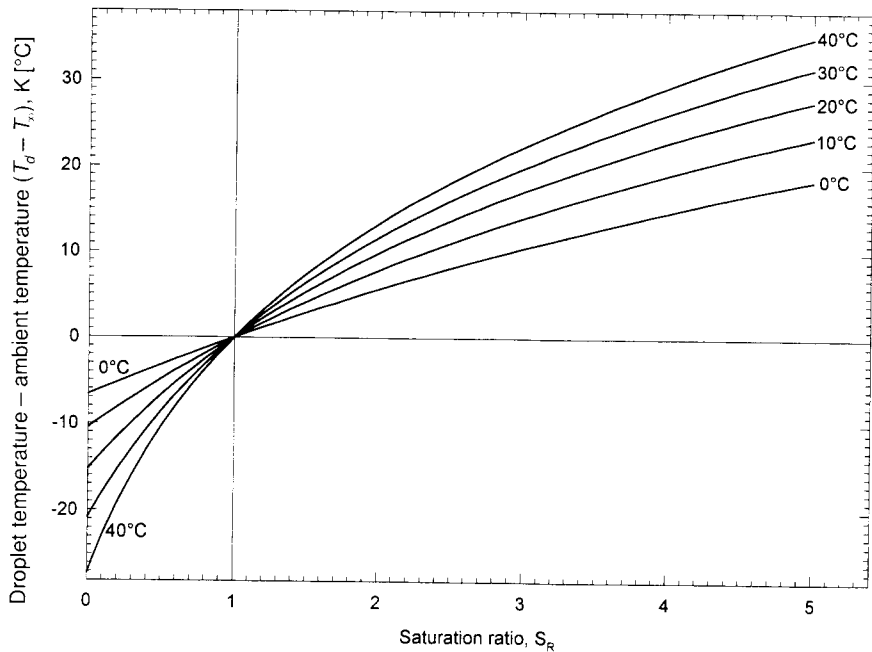
FIGURE 13.3 Water droplet temperature–ambient temperature ( T_d - T_x ) versus saturation ratio for ambient temperatures of 273–313 K [0–40°C].
