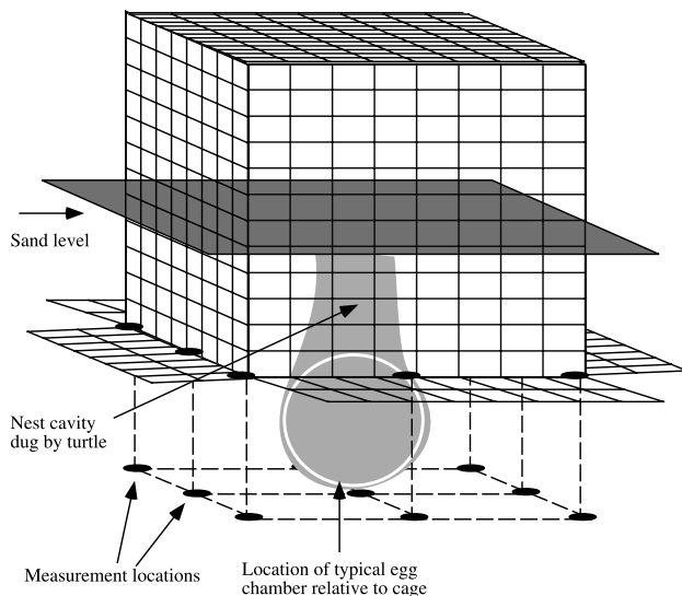
Fig. 1. Diagram of a protective wire cage and measurement locations. Measurements of the magnetic field were made 25 cm beneath each cage at a series of locations; these included sites below the center, each corner and the mid point of each side and immediately below each cage at the same 9 points. Galvanized wire protective cages are placed approximately 25 cm deep in the sand over a turtle nest. The measurement depths therefore corresponded to the average top and bottom of a loggerhead egg chamber (Dodd, 1988).
