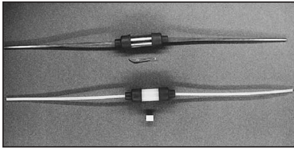
FIGURE. Top: 40-cm-long and 3-mm-diameter stainless steel lumen test unit with stainless steel surgical-blade carrier. Once inoculated, the blade is aseptically placed in the removable center portion by unsealing the hard rubber septums connecting the stainless steel tubing. Bottom: 40-cm-long and 3-mm-diameter plastic lumen test unit with porcelain cylinder carrier. Once inoculated, the carrier is aseptically placed in the removable center portion by unsealing the hard rubber septums connecting the plastic tubing.
