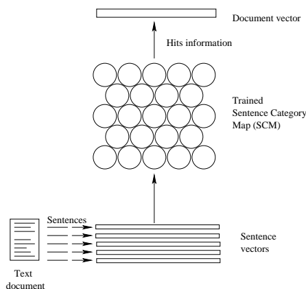
Figure 2: Extending document vectors
