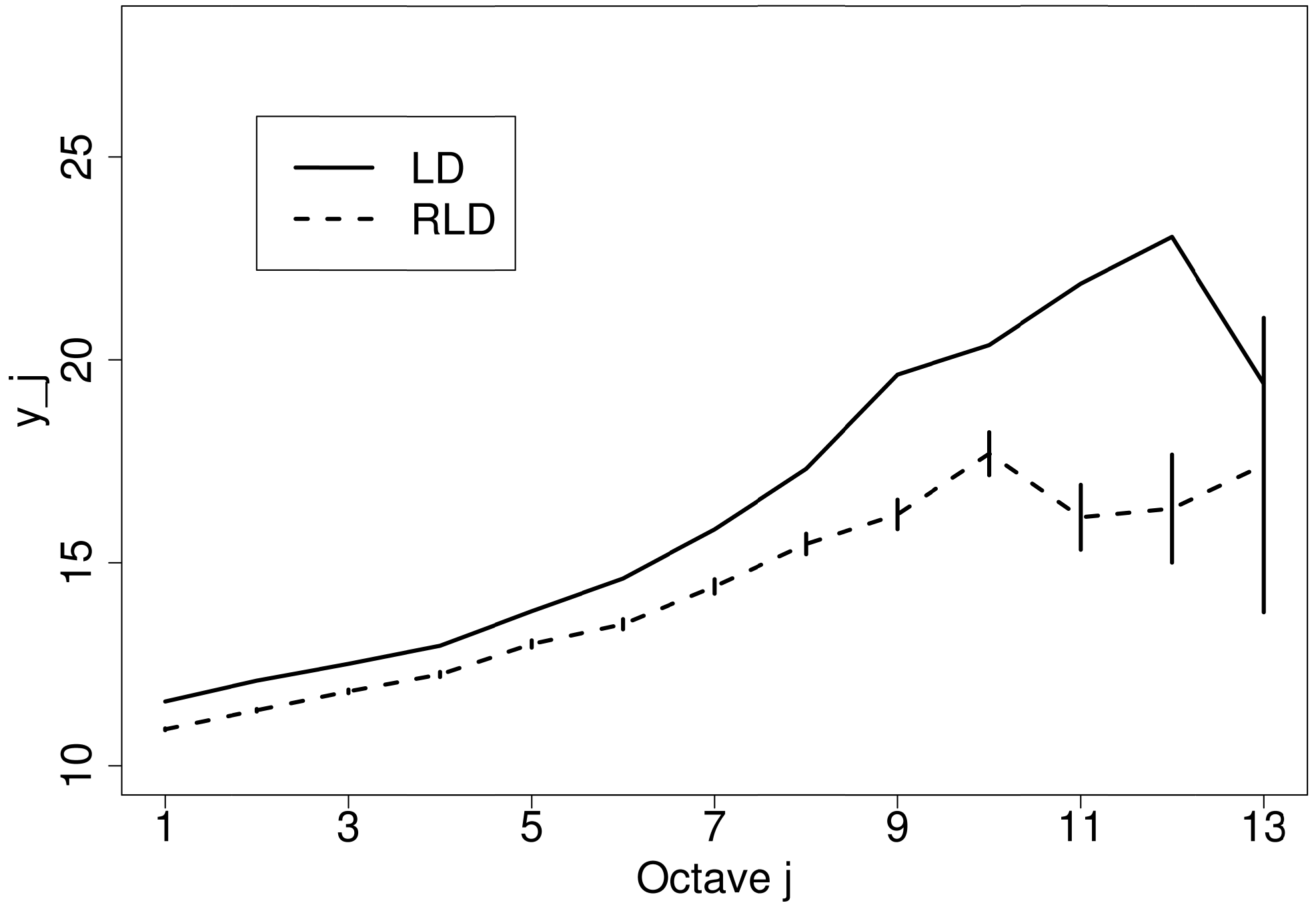
(b) UNC02-APR-09: Logscale Diagram
