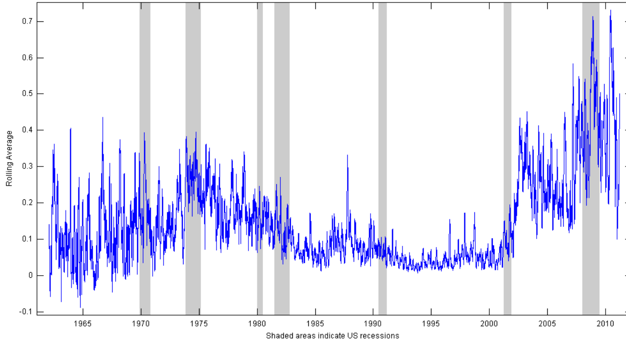
Rolling Average Correlation Coefficient for S&P 500 Period = 20 Days Updated: 3/25/2011
