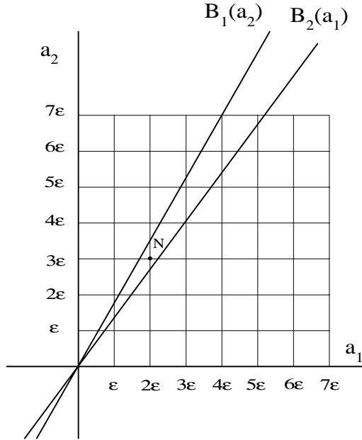
Figure 1: Nash Equilibria of a Discretized Game.
