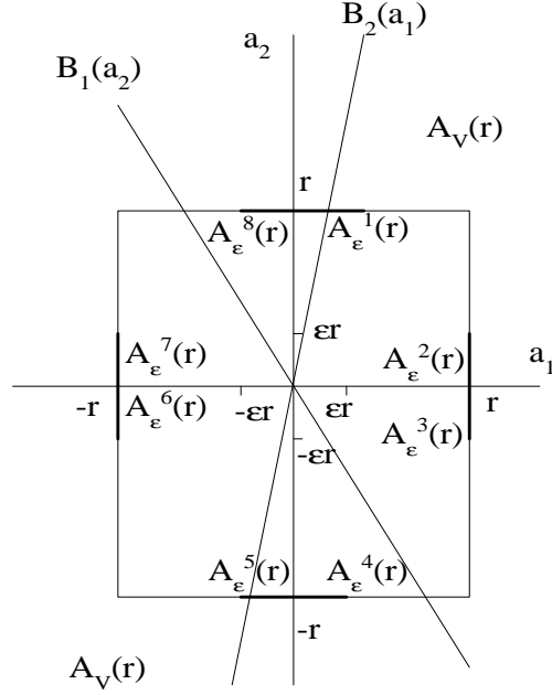
Figure 2: The set A(r) = \{a \in A : \rho(a) = r\} .
