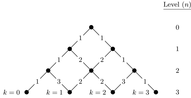
Fig. 1. The first three levels of the Euler graph. The numbers on the diagonals give the number of edges coming out of each vertex, and k represents the label on each vertex.
