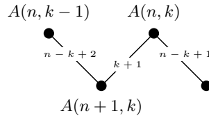
Fig. 2. The Euler Graph gives rise to Equation 1-1.
