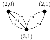
Fig. 3. The order on the edges coming into vertex (3,1) : e_0 < e_1 < e_2 < e_3 < e_4 .
