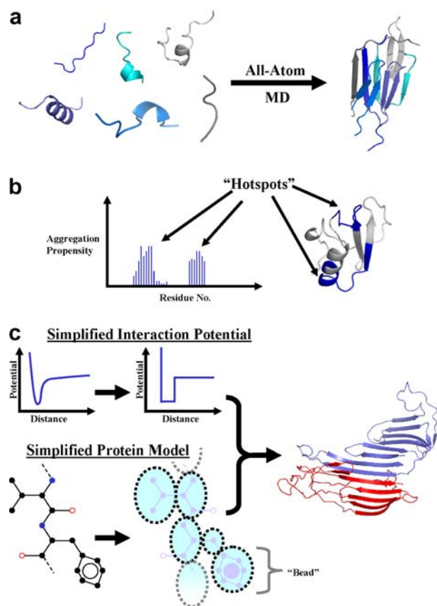
Fig. 5. Computational studies of protein self-association and aggregation. Different computational techniques have been utilized to study various aspects of protein self-association and aggregation. (a) All-atom molecular dynamics is used to model the aggregation of short peptides. (b) Simulations of peptides from within larger proteins are used to suggest aggregation “hotspots”. (c) By combining simplified interaction models and protein models, aggregating systems that are inaccessible by traditional molecular dynamics due to size and time limitations can be studied. The curves show the approximation of a continuous interaction potential by a square well as used in DMD [58]. The dotted circles represent “beads” in the model which take the place of several atoms in the original protein. The structure to the right shows the self-association of two identical proteins forming an extended \beta -sheet.
