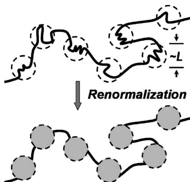
Fig. 4. Unfolded protein states. The unfolded state of a protein features residual local structures, which span a short segment of approximately 10 residues ( L \sim 10 ). This structural correlation quickly decays as the segment length increases. A renormalization process, which groups the local amino-acid residues into a coarse-grained bead, reduces the unfolded protein into an effective non-interacting polymer.
