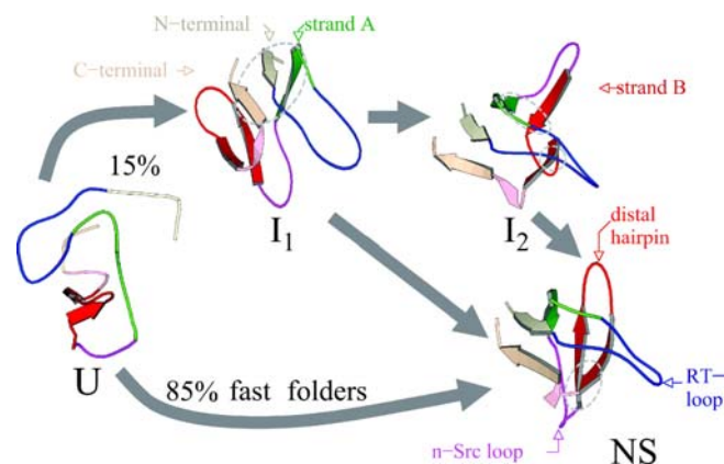
Fig. 2. Fast and slow folding pathways. Molecular dynamics simulations of the c-Crk SH3 folding show multiple folding pathways via only one or two intermediates. [Reprinted with permission from Ref. [258]. Copyright Biophysical Society.]
