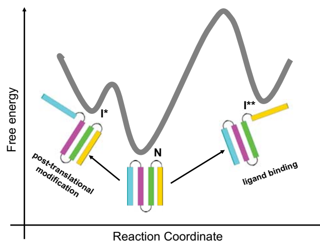
Fig. 3. Protein intermediate states. Intermediate states are meta-stable in protein free-energy landscapes ( N : the native state; I^* , I^{**} : intermediates). They may play a significant role in protein function, including exposing cryptic post-translational modifications or ligand binding sites.
