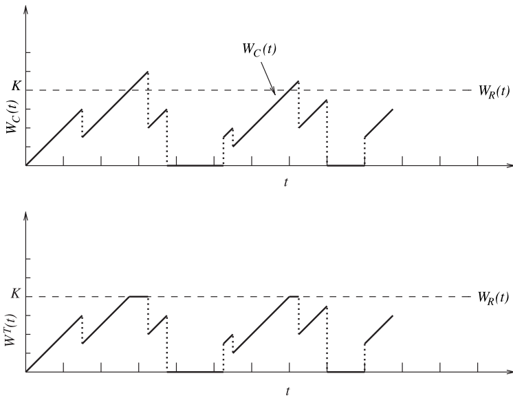
FIGURE 3. Sample paths of W_C(t) and W(t) in the presence of time-outs.
