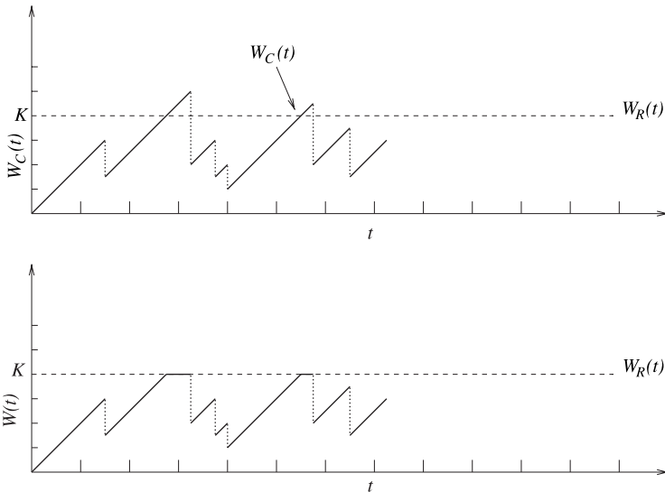
FIGURE 1. Sample paths of W and W_C processes in the absence of time-outs.
