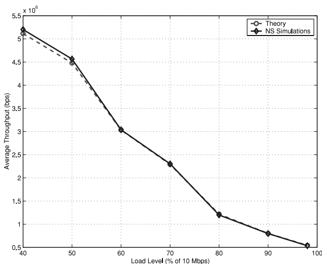
FIGURE 4. Throughput comparison.
