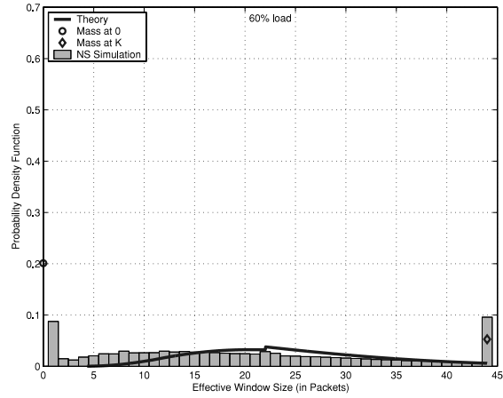
FIGURE 7. Comparison of effective window-size distributions at 40%, 50%, and 60% loads.
