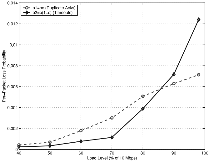
FIGURE 5. Loss rates in NS simulations.
