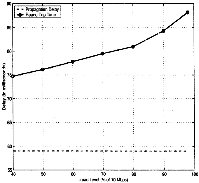
FIGURE 6. Mean RTTs in NS simulations.
