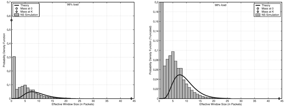
FIGURE 9. Comparison of effective window-size distributions at 98% loads.
