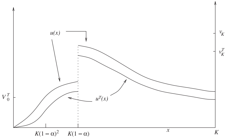
FIGURE 2. Typical graph of the density u and u^T of the window size.
