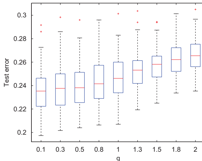
Fig. 4. Plot of classification errors in Example 1 as q increases.
