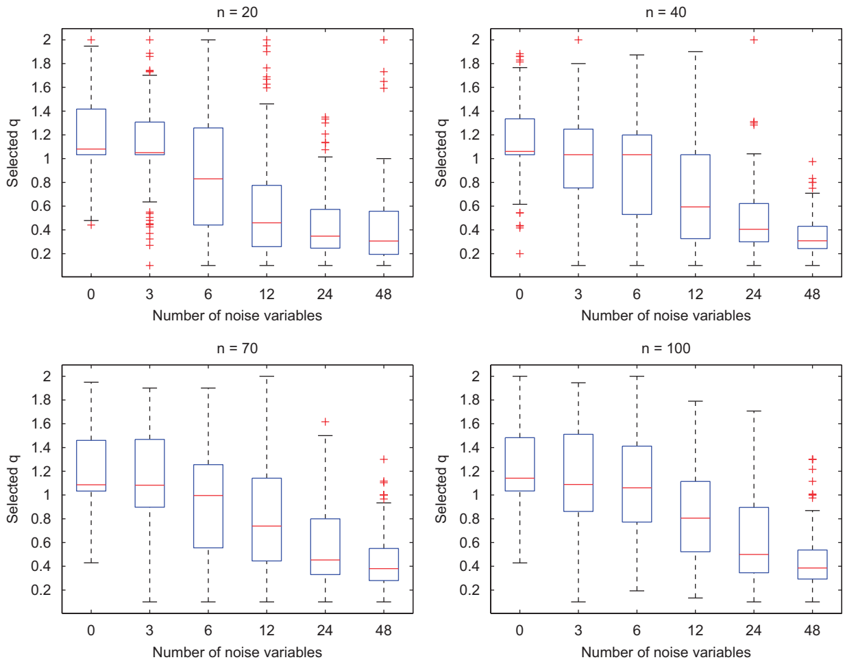
Fig. 6. Plot of best selected q 's in Example 2 as the numbers of noise variables increase.
