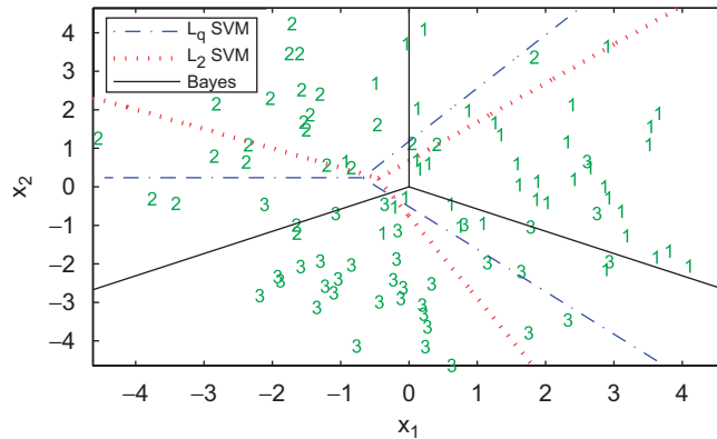
Fig. 9. Classification boundaries given by the Bayes rule, the L_2 , and L_q SVMs in Example 4.
