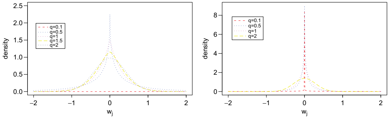
Fig. 2. Plots of the density function \pi_{\lambda,q}(w_j) with \lambda = 3 (left panel) and 6 (right panel).
