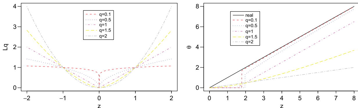
Fig. 1. Plots of L_q penalties with different q 's (left panel) and the corresponding solutions \hat{\theta} = \arg \min_{\theta} F_q(\theta) (right panel) with \lambda = 3 , where F_q(\theta) = (\theta - z)^2 + \lambda|\theta|^q .
