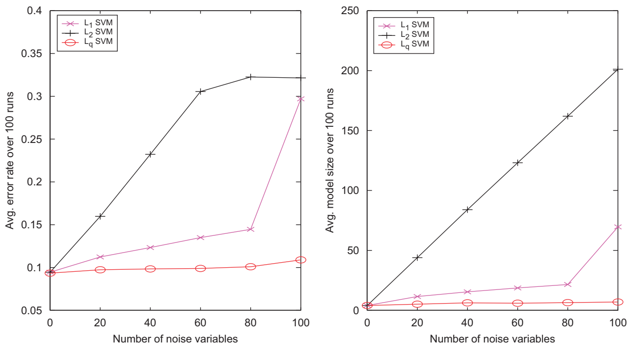
Fig. 7. Plots of average misclassification rates and model sizes for Example 3 over 100 runs.
