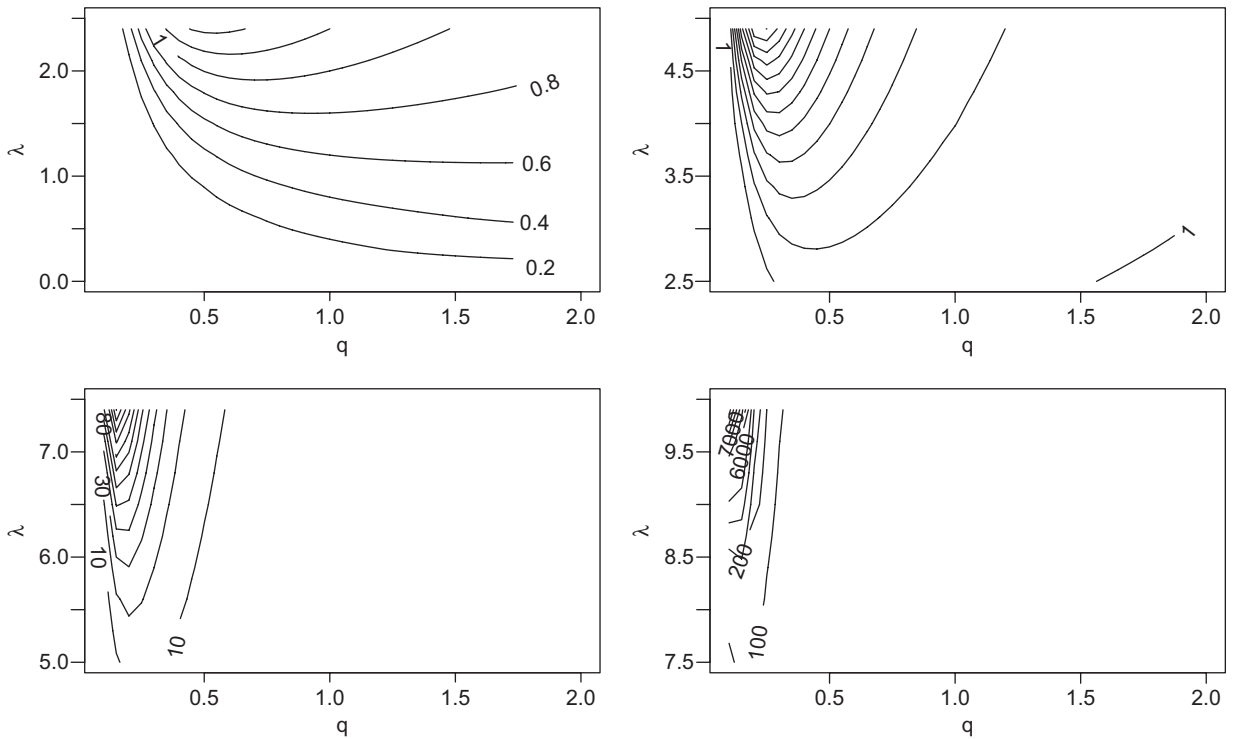
Fig. 3. Contour plots of the density coefficient q\lambda^{1/q}/2\Gamma(1/q) in (2) with q \in (0, 2] and \lambda \in (0, 10) .
